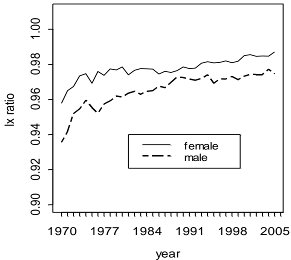
France (1970-2006)
