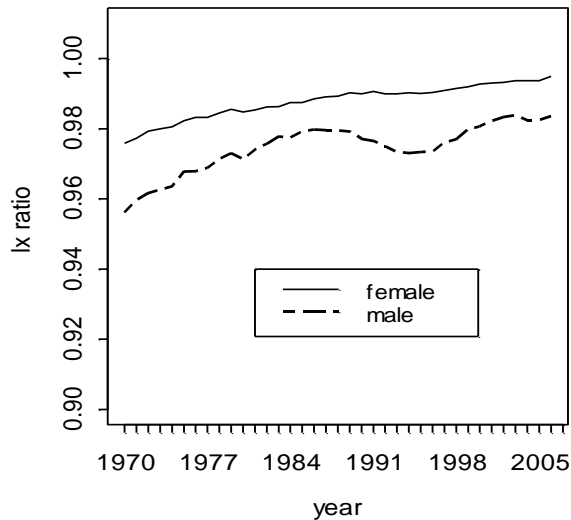
England & Wales (1970-2006)
