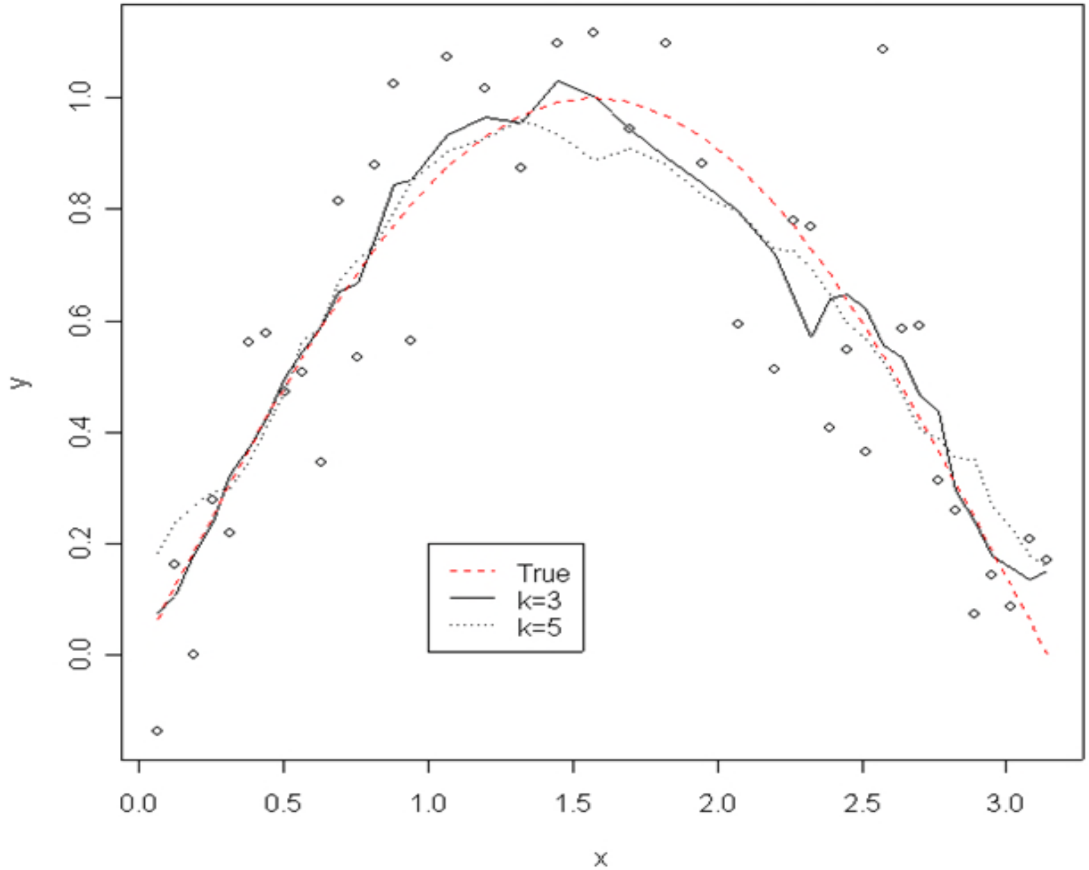
Running means ( y=\sin x )
