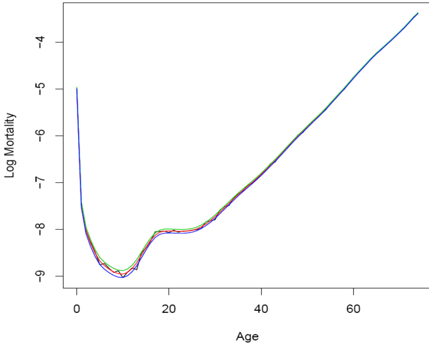
Figure 1 Raw Data (Black), Upper 95%, Lower 95% and Bayes Estimate.
