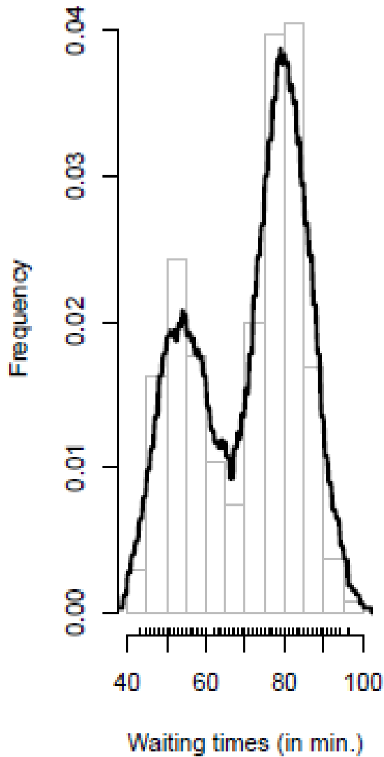
Rectangular kernel
