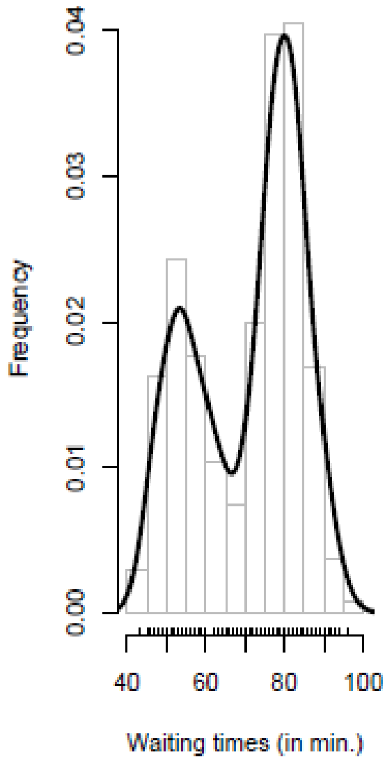
Gaussian kernel
