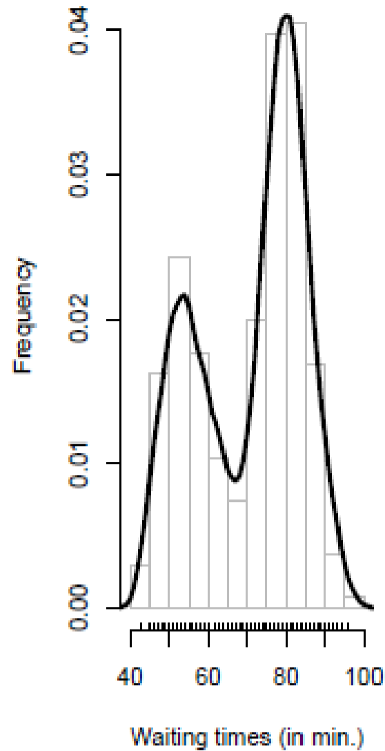
Triangular kernel
