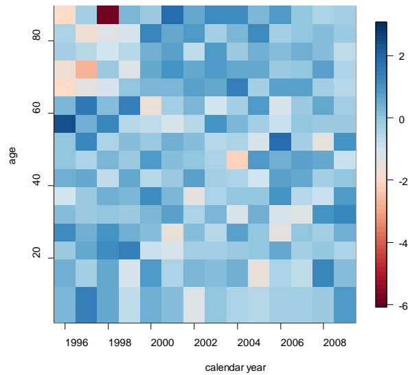
Figure 4. Residuals of the LC model (Cancer, Male)
