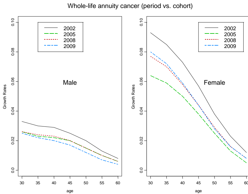
Figure 8. % Difference in pure premium whole-life annuity cancer (LC Model)
