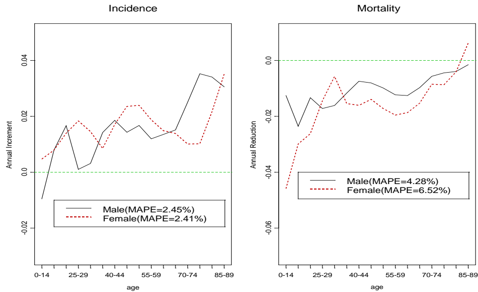
Figure 6. Annual increment/reduction of cancer data (LC Model)
