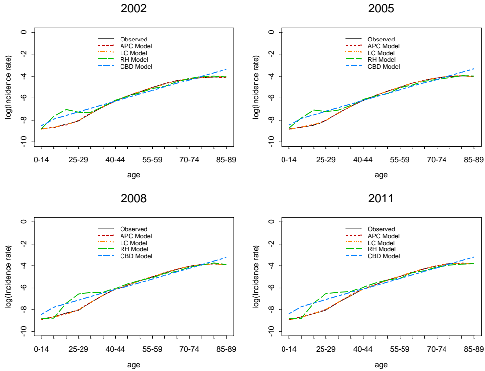
Figure 5. Observed vs. estimated cancer incidence rates (Male)
